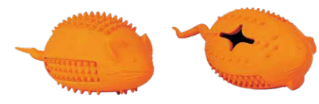
Item:066070 Material:Natural Rubber Weight:101g Size:100*58*58mm
